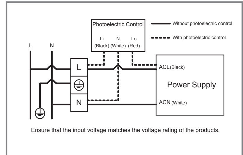
Wiring diagram
