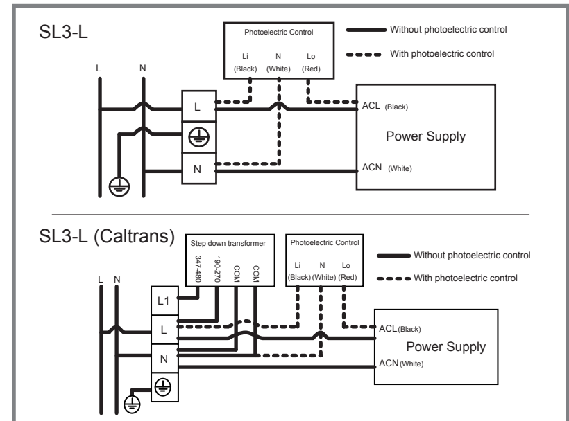
Wiring diagram
